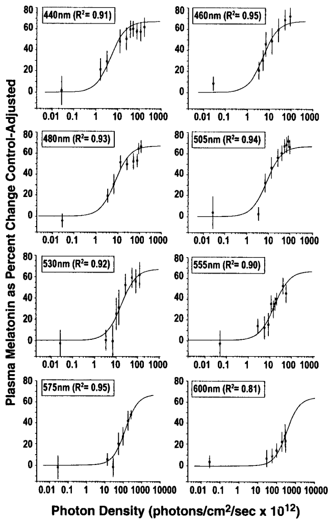
Figure 3. This figure illustrates the fitted univariate fluence–response curves for monochromatic light exposures and percent control-adjusted melatonin suppression for eight wavelengths of visible light. Each fluence–response curve is derived from eight healthy volunteers who participated in a complete, within-subjects experimental design. In each graph, the data points represent group means \pm SEM. Each curve has a high coefficient of correlation (0.95–0.81).
